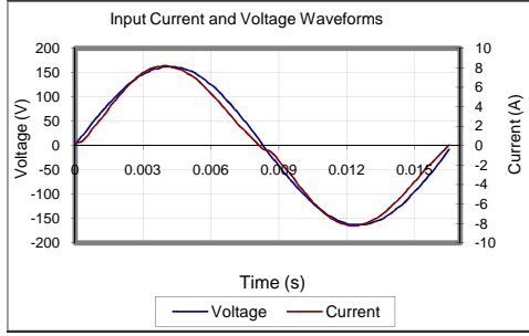
Input AC Current Waveform (ITHD = 9.05%, 50% Load)
