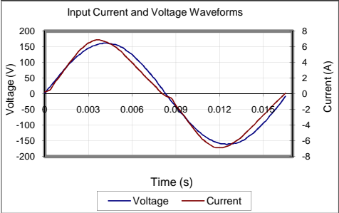
Input AC Current Waveform (ITHD = 11.61%, 50% Load)
